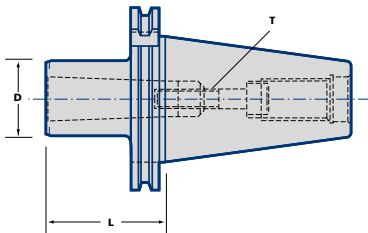
Fig 2 DRAWBOLT TYPE - MB
