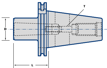
Fig 3 COMBINATION TYPE - MC (TANG and DRAWBOLT)
