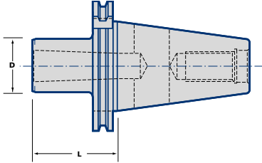
Fig 1 TANG TYPE - MT
